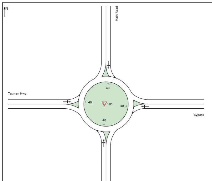
Figure 6.3: Tasman Highway/Southern Sorell Bypass/ Main Road / Giblin Drive Roundabout Layout
