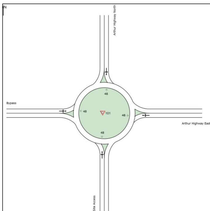
Figure 6.1: Growth Area Access/Arthur Highway/Sorell Southern Bypass Roundabout Layout
