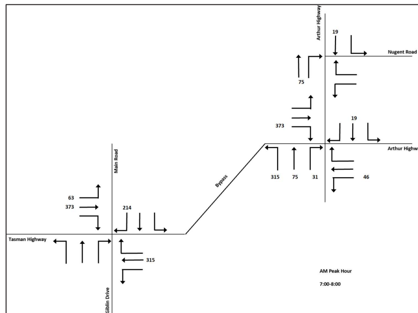
Figure 5.3: 2042 Growth Area Generated AM Peak Hour Traffic Volumes (Full Development)
