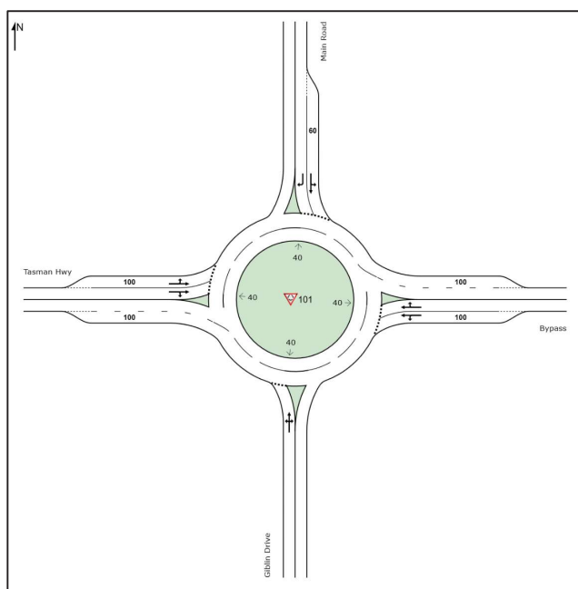
Figure 6.4: Tasman Highway/Southern Sorell Bypass/ Main Road / Giblin Drive Duplicated Roundabout Layout
