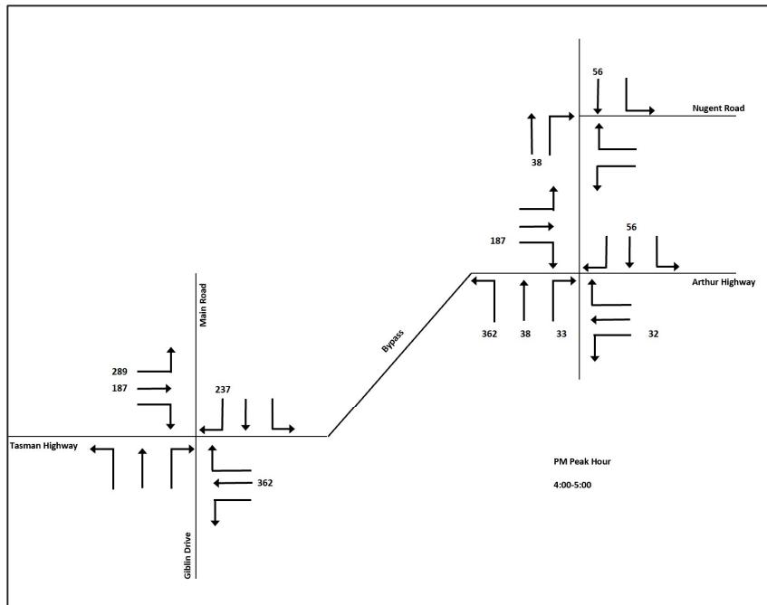
Figure 5.4: 2042 Growth Area Generated PM Peak Hour Traffic Volumes (Full Development)
