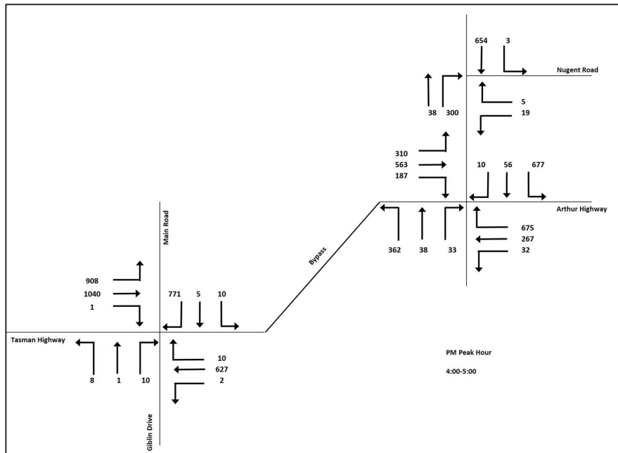
Figure 5.6: 2042 Ultimate PM Peak Hour Traffic Volumes
