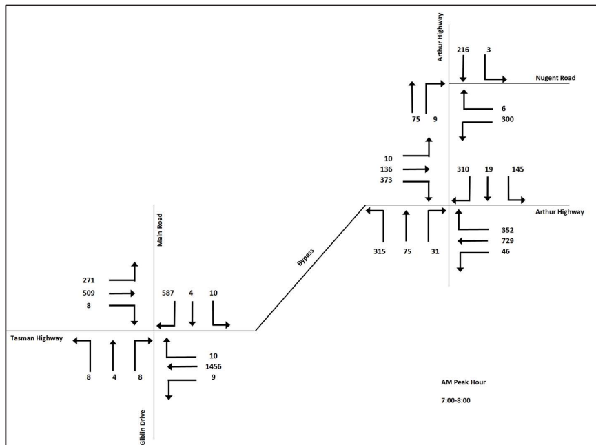
Figure 5.5: 2042 Ultimate AM Peak Hour Traffic Volumes
