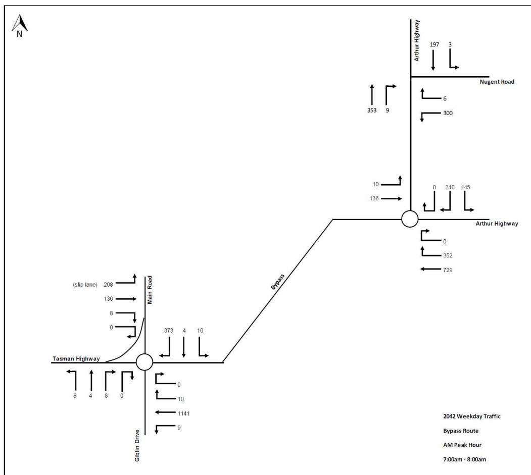
Figure 5.1: 2042 Weekday Background Volumes (AM Peak)
