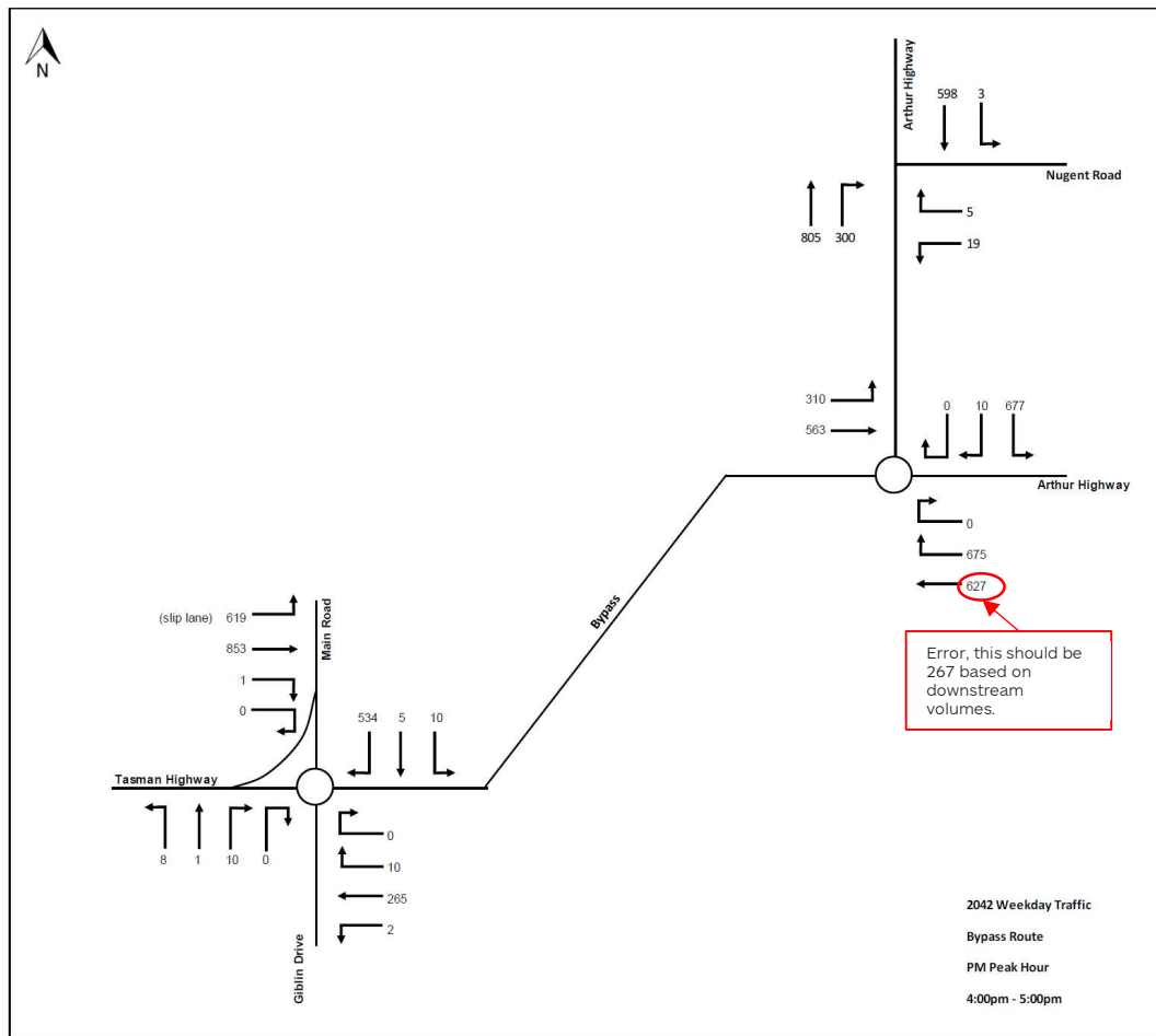
Figure 5.2: 2042 Weekday Background Volumes (PM Peak)
