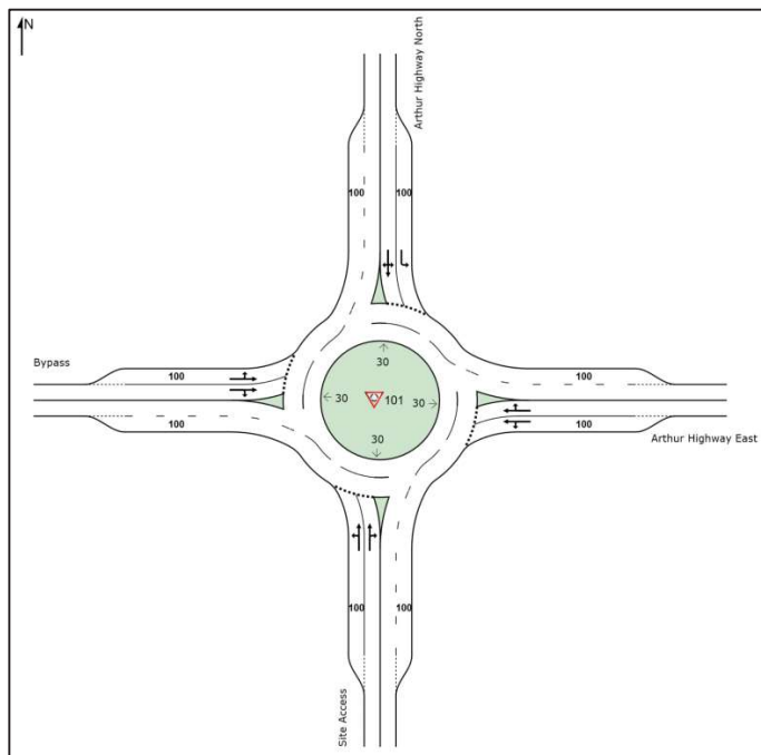
Figure 6.2: Growth Area Access/Arthur Highway/Sorell Southern Bypass Duplicated Roundabout Layout
